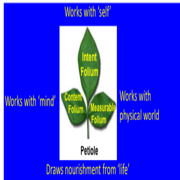
Fig. 1. Geometry of Information: Information connects physical/material plane with the mind and self. It could do so because of its specific geometry. Information is like a trifoliate leaf of which the measurable folium interacts with physical world, content folium interacts with mind world and intent folium interacts with 'self'. The petiole of leaf gets nourishment from 'life'. The strength of mind comes from 'life'. Information has no direct access to consciousness.
