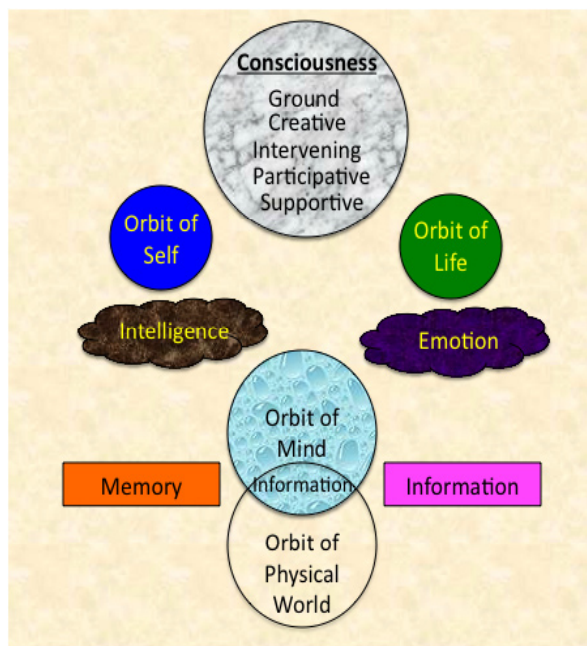
Fig. 2. Tentative localization of the operational orbits of the nonlocal constituents of systems psyche: The orbit of consciousness is at the bottom of the depth. Consciousness also works in layers. Next begins the nature at nascent stage where the operational orbits of 'self' and 'life' could be located. This is sub-sub-quantum plane of nature. Superficial to this is the plane of emergence of intelligence and emotion, and more superficially are the orbits of operation of mind, memory and information. All are constituents of sub-quantum nest of nature. The orbit of operation of mind intercepts with the orbit of physical world. Physical world and mind world are connected through signal-information transformation.
